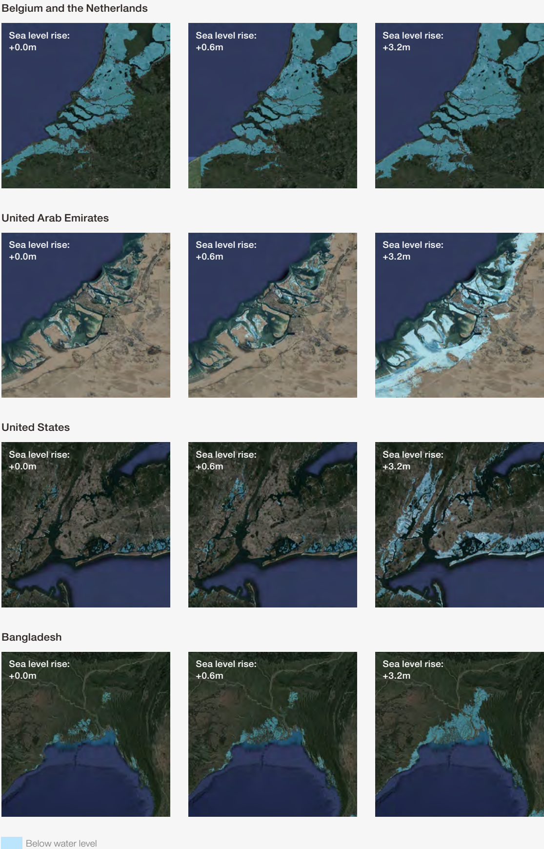
FIGURE 2.9 | Indicative sea level rise, selected countries
